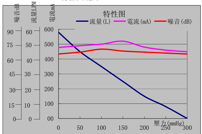
特性曲綫圖 Characteristic Curve:
